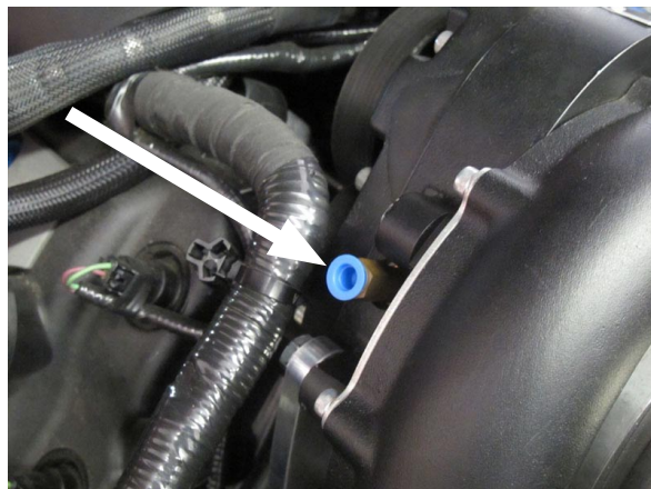
Fig. 13A: Supercharger Oil Feed Location
