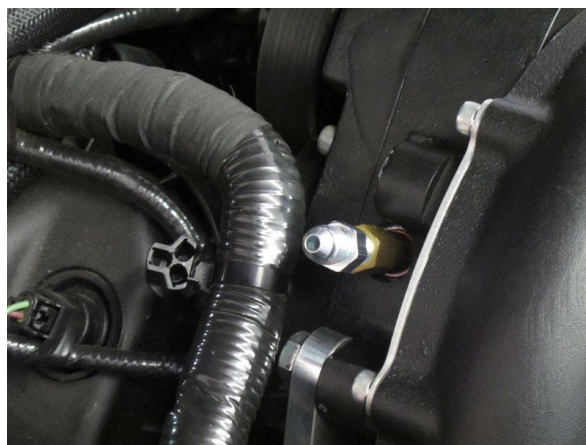
Fig. 13B: -4AN Oil Feed Fitting Installed
