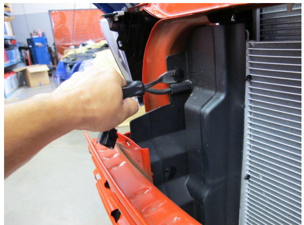
Fig. 1L: Radiator Side Shroud, Passenger ('11-'12 Mustang)
