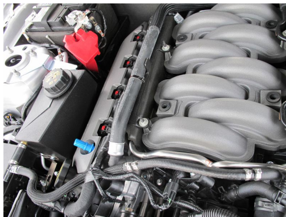
Fig. 3X: 5/16" Coolant Hose, Extended
