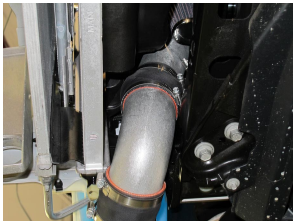
Fig. 7B-2: 90° Tube and Bump Coupler
