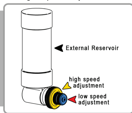
TQ Series (3 possible adjustments) Single rebound like the HQ Series Dual stage compression adjustment
