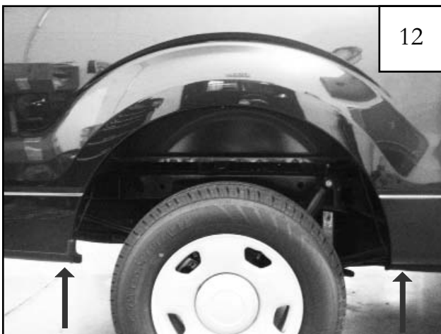
Remove two factory bolts with a 10mm socket wrench. (Note: New hardware is being supplied see Step 17)
