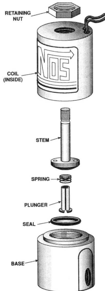
Exploded View of a Typical Solenoid
