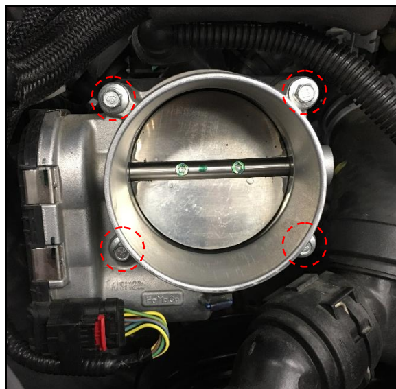
Figure 9 – Throttle Body Removal
