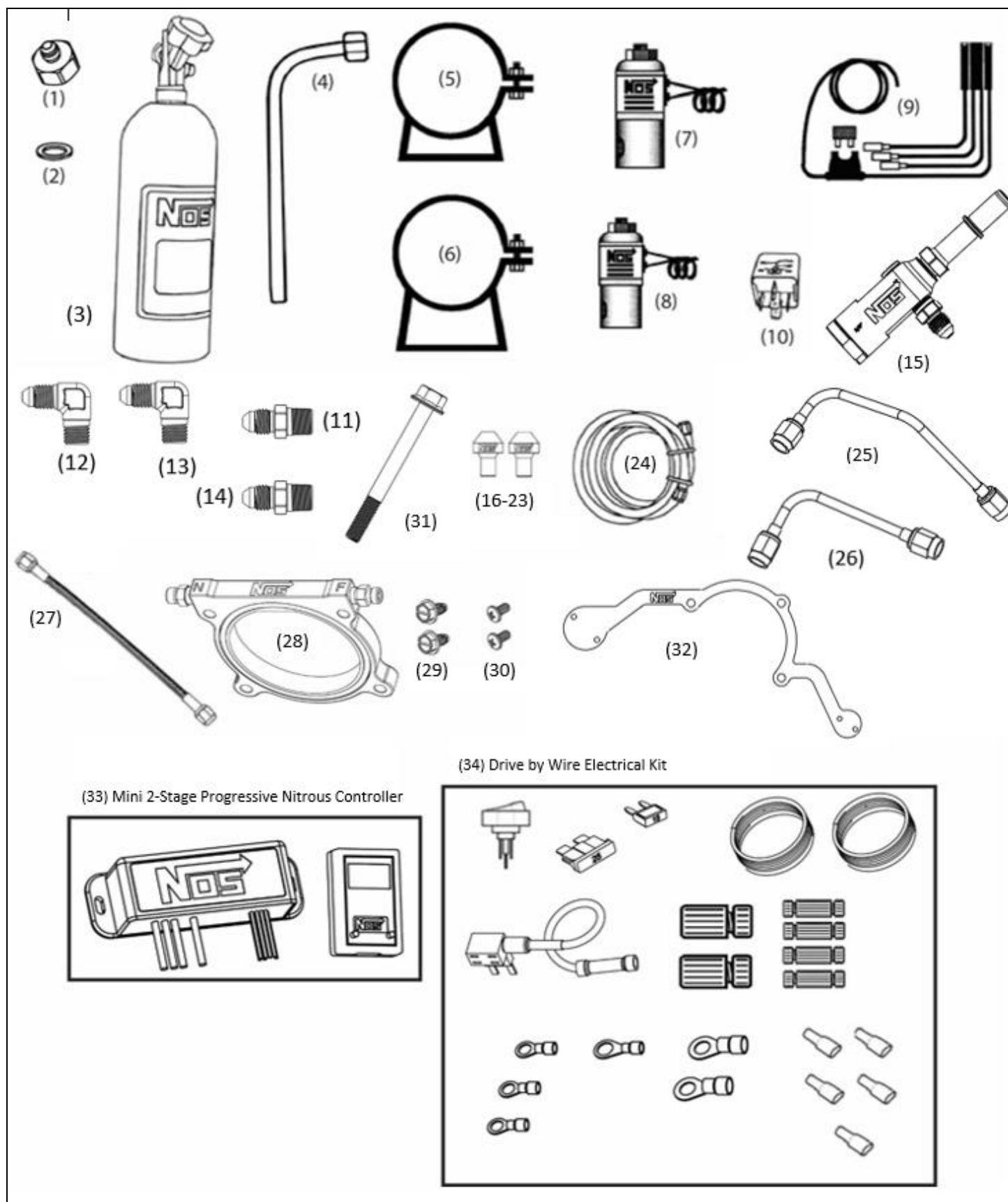
Figure 1 Kit Number 02127NOS & 02127BNOS Component Identification
