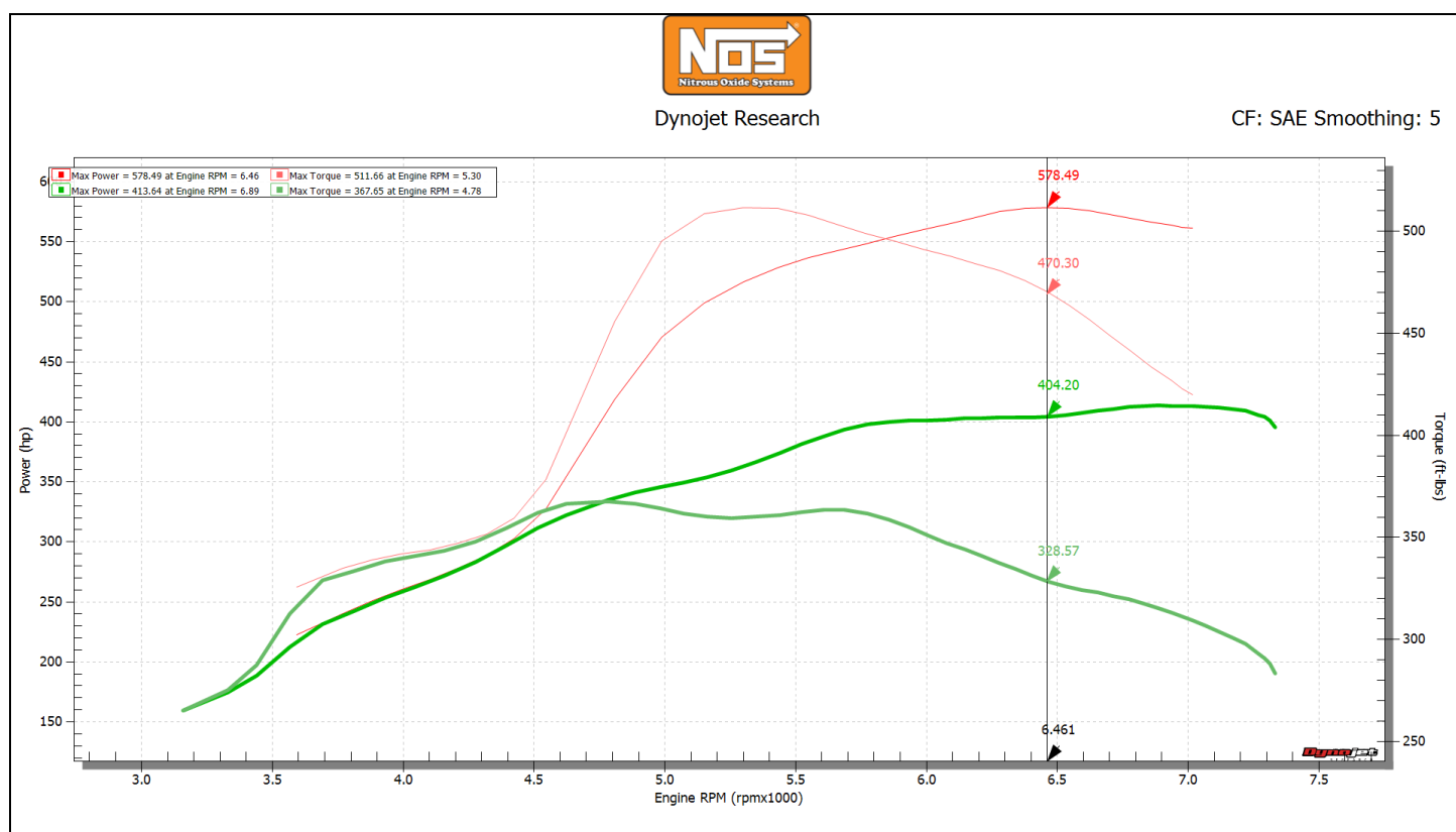
Figure 21 – 175HP Shot Dyno Graph
