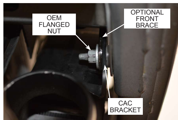
Fig. 5-c: CAC Installation - Vehicles w/ Front Braces
