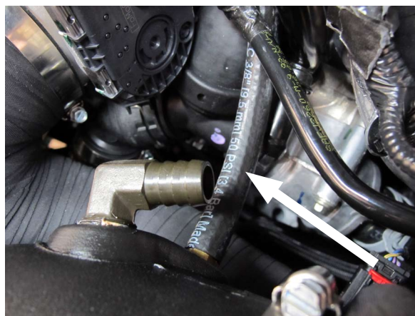
Fig. 8-l: 3/8" Hose From Tee To 3/8" Air Inlet Barb
