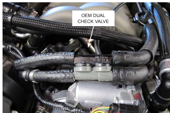
Fig. 8-k: 3/8" Hose Attachment
