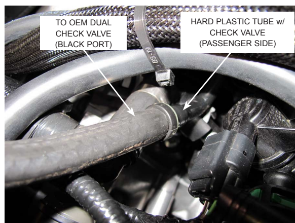
Fig. 8-j: 3/8" Hose - Hard Plastic Tube (Passenger Side)
