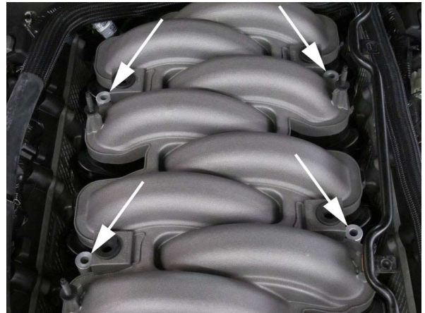
Fig. 6-d: Aluminum Fuel Rail Spacers
