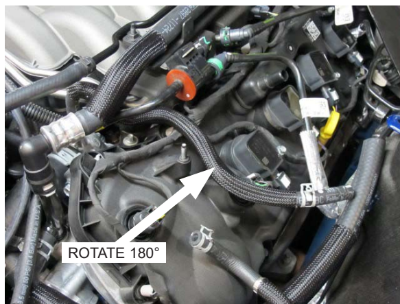
Fig. 3-n: Rotate Upper OEM Molded Coolant Hose 180° (Rotated View Shown)
