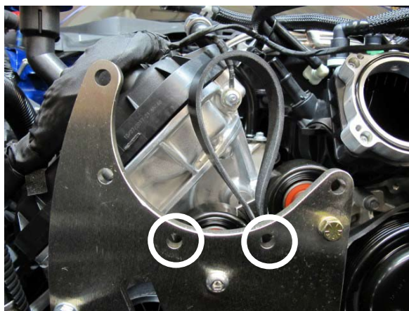
Fig. 2-o: Use long 9/16" Wrench To Install These Screws
