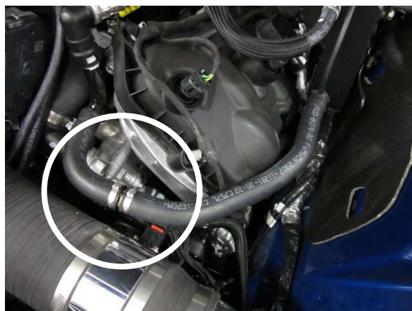
Fig. 3-v: OEM 3/4" Coolant Hose (Modified)
