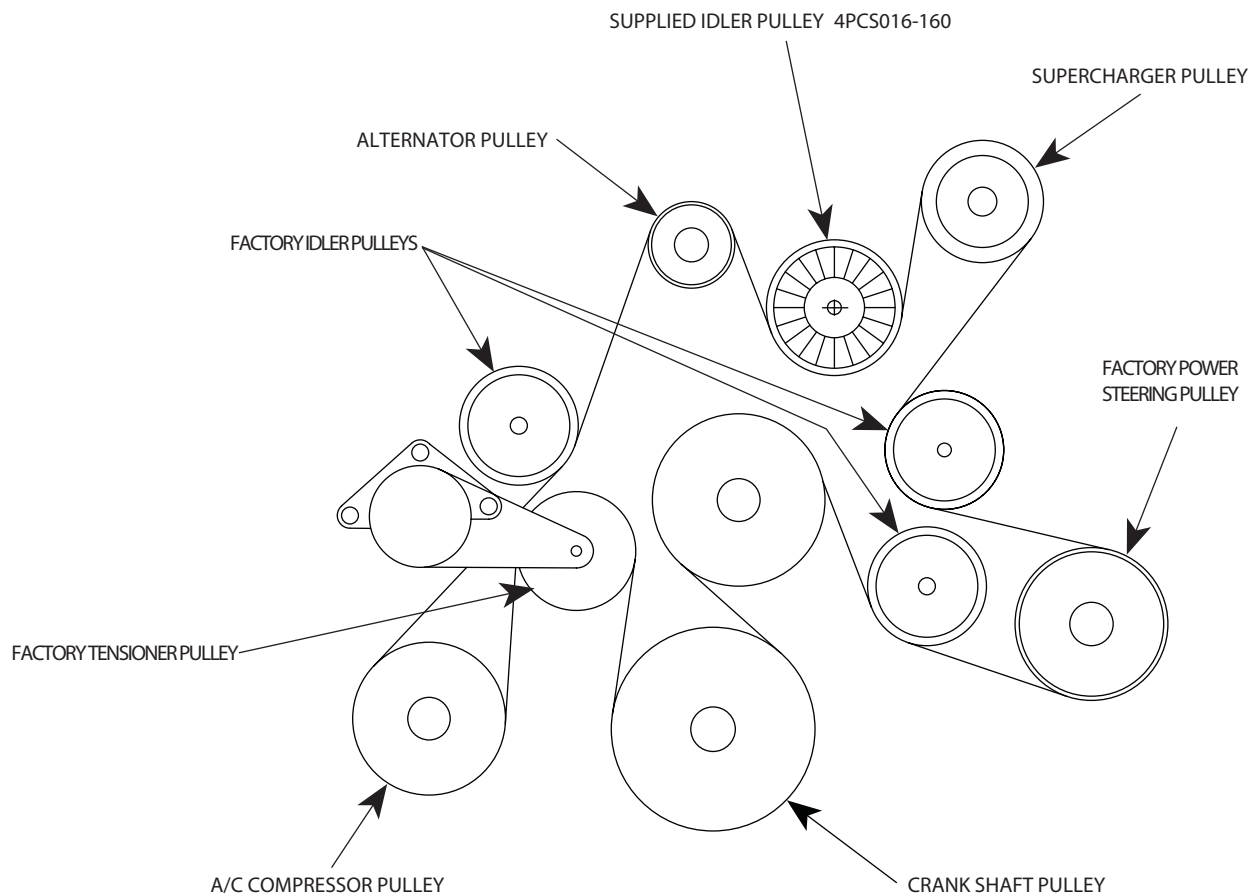
Fig. 6.2-e / Belt routing
