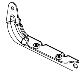
Link Control Bracket Left Part #598.19 Qty. 1
