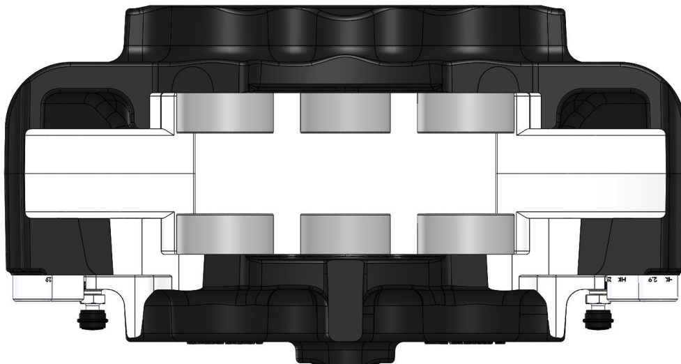
Fig 1 – Caliper pistons moved forward to facilitate removal
