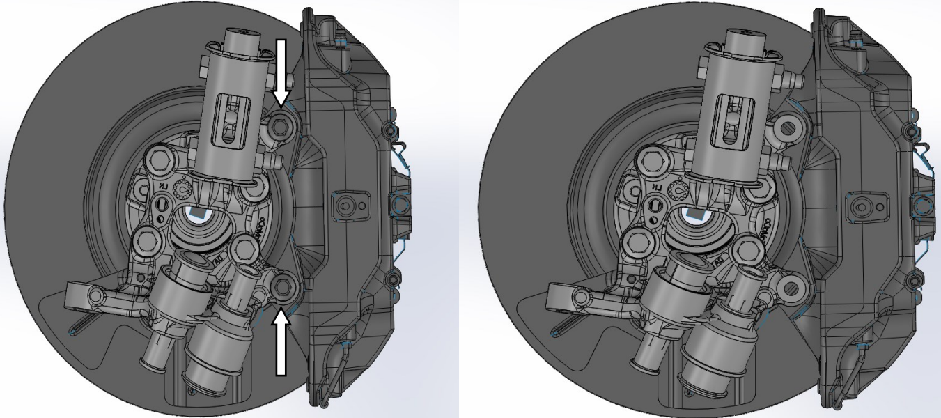
Figure 1. Caliper retaining hardware removal
