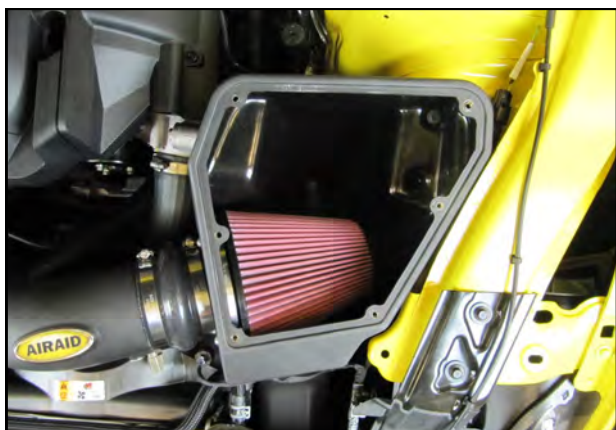
18. Install the Airaid Premium Filter onto the Filter Adapter inside of the Airbox.
