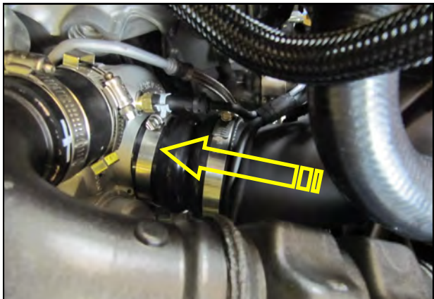
15. Lower the Airaid Intake tube down into position and slide the reducer onto the turbo inlet.
