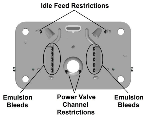
2 Circuit Billet Metering Block (Front) Model 4150 ALUMINUM Figure 10
