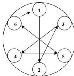
Proper torque sequence for cover bolts
