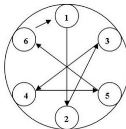
Proper torque sequence for cover bolts
