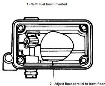
External Adjustable Type FIG. 2 - DRY FLOAT SETTING
