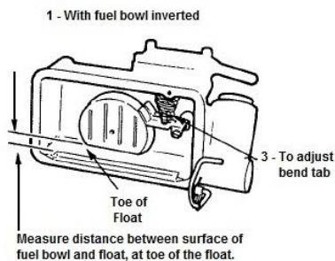
Non-Adjustable Type FIG. 4 - DRY FLOAT SETTING
