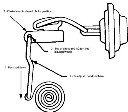
FIG. 9 - CHOKE ROD ADJUSTMENT
