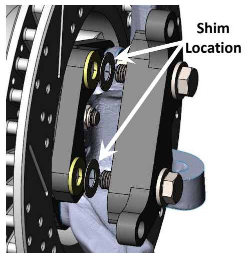
Figure 7c - Shim Location
