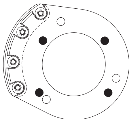
Figure 1. Wilwood Caliper Mounting Bracket
