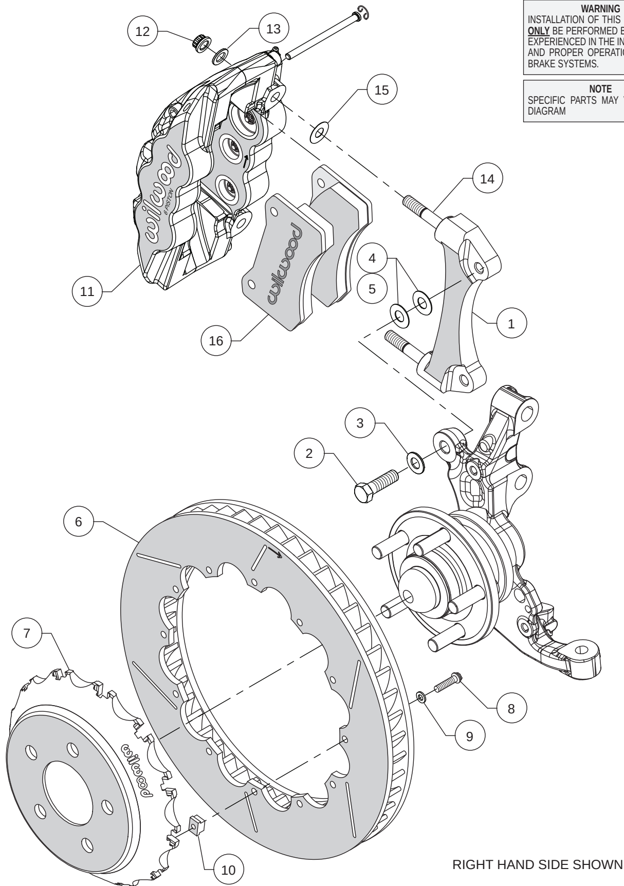
Figure 1. Typical Installation Configuration
