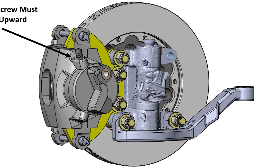
Figure 7 - Caliper Installed (Passenger Side Shown)
