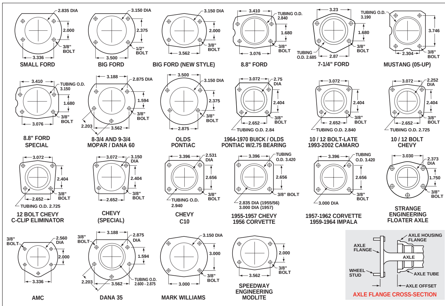
Figure 5. Rear Housing Flange Chart and Axle Flange / Offset Cross-Section
