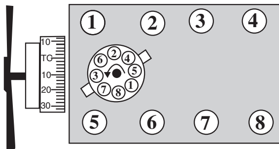
Figure 2 - 351-M/400 c.i.d. Ford V8 Firing Order 1-3-7-2-6-5-4-8 Turn distributor clockwise to advance timing.
