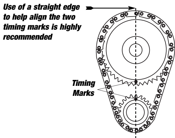
Figure 1 Timing Chain Sprocket Alignment & Timing Marks
