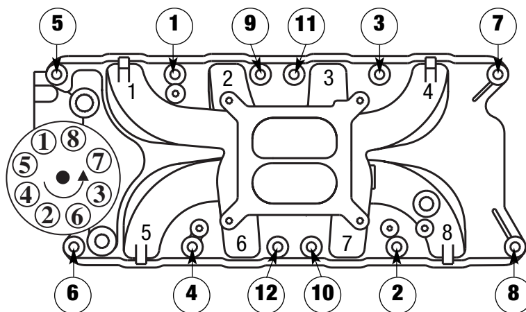
Figure 2 - 260-289-302 Ford Torque Sequence Torque Bolts to 18-20 ft/lbs.
