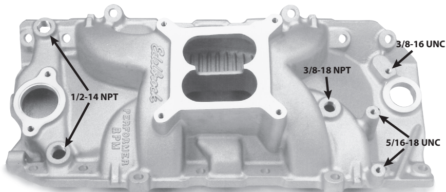
Fitting Boss Thread Sizes (Depending on application, not all bosses will be present)
