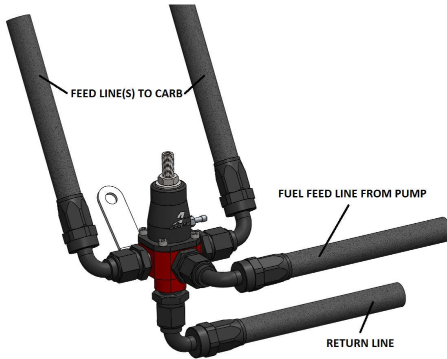
CONVENTIONAL CARB PLUMBING
