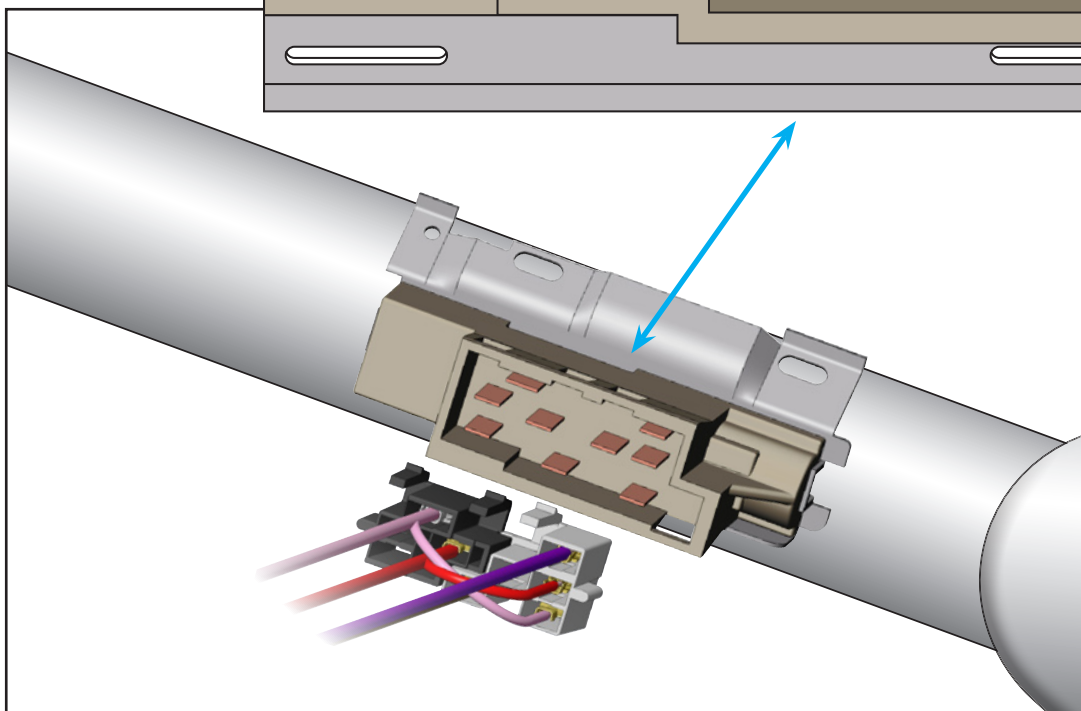
IGNITION SWITCH DETAIL
