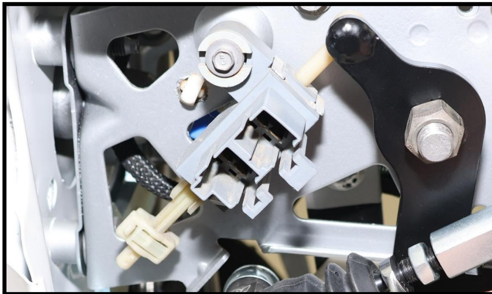
MDL Clutch pedal with carriage bolt/nut, and neutral start switch.
