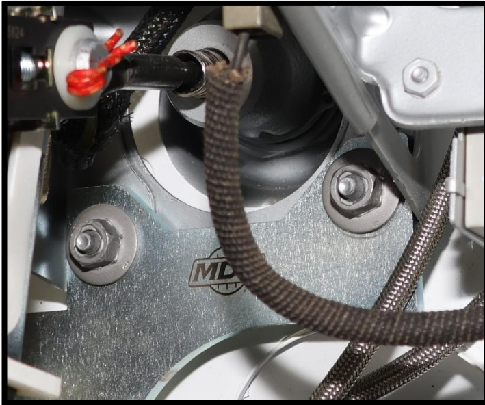
Bracket shown installed on booster studs.
