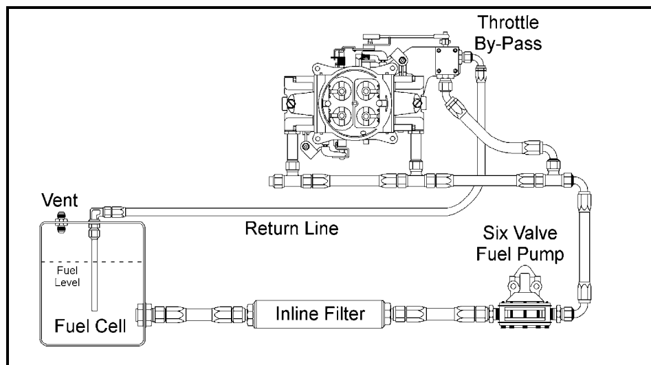
Throttle By-Pass System with Six Valve Fuel Pump
