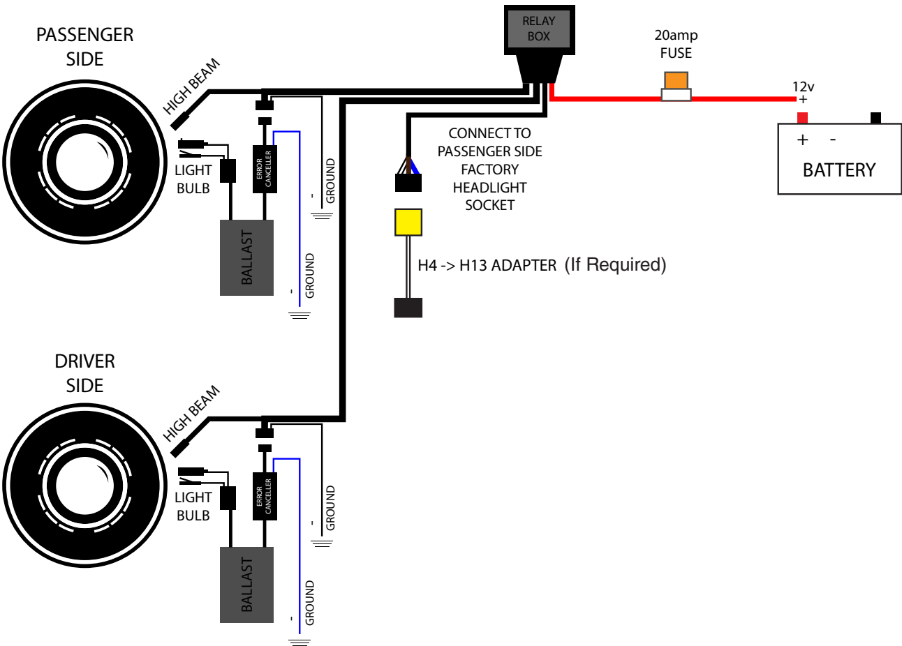
FIGURE 1 WIRING HARNESS
