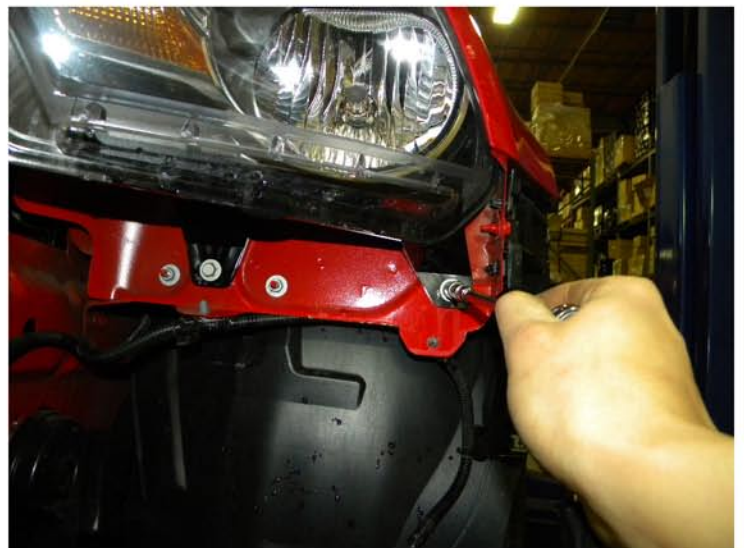
16. Remove the (2) 10mm bolts
