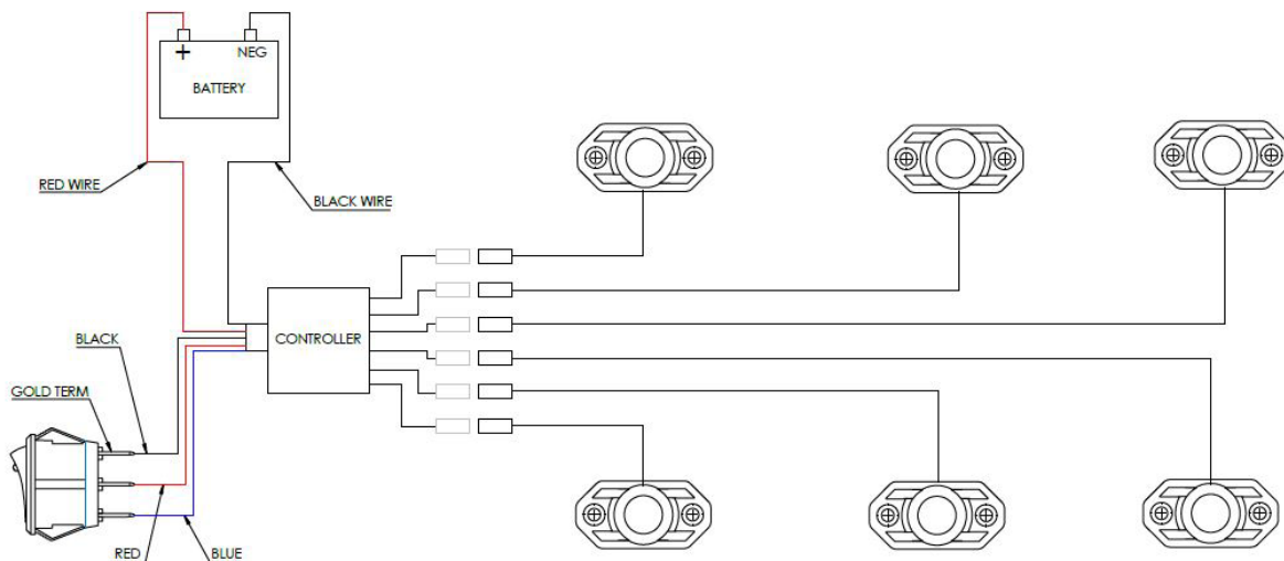
Wiring diagram
