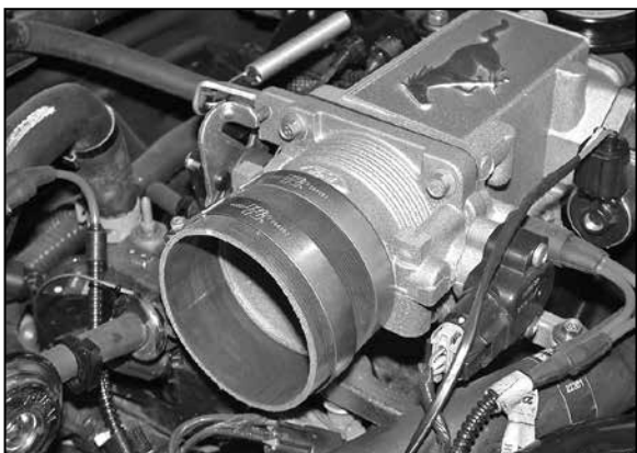
15. Install the provided silicone hose and hose clamps onto the throttle body as shown.
