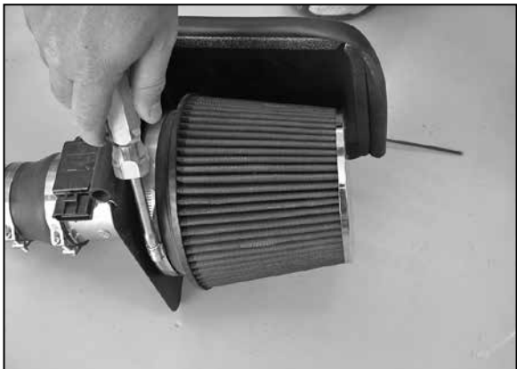
20. Install the K&N® air filter onto the filter adapter and secure with the provided hose clamp as shown.
