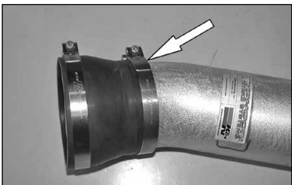
18. Install the provided silicone step hose and hose clamps onto the K&N® intake tube as shown.
