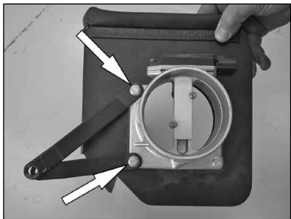
14. Attach the brackets to the mass air sensor flange as shown.
