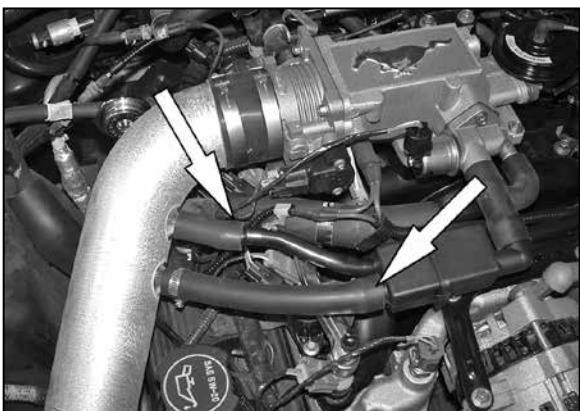
23. Reconnect the vent hoses to the K&N® intake tube as shown and tighten hose clamps.
