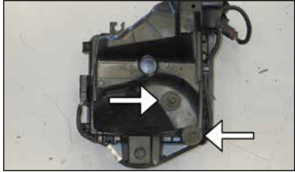
13. Remove the two airbox mounting grommets from the factory airbox.
