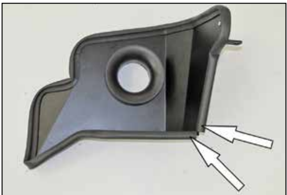
13. Install the provided edge trim onto the heat shield as shown. NOTE: Some trimming of the edge trim will be necessary.
