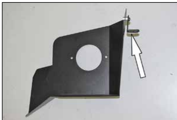
11. Install the provided heat shield mounting bracket (064326) onto the heat shield as shown using the provided hardware. NOTE: Be sure to place the provided spacer between the bracket and heat shield.
