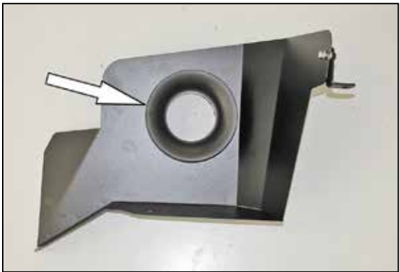
12. Install the provided filter adapter into the heat shield as shown and secure with the provided hardware.
