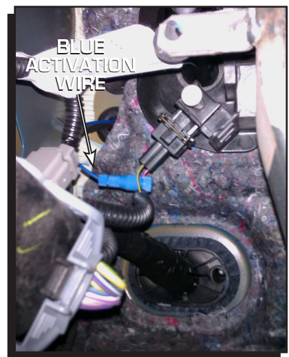
Figure 4 Activation Wire.
