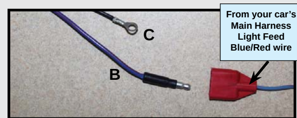
Figure 1-B: Black wire ground to chassis (C) Blue wire with red stripe connects to instrument panel light circuit lead. (B)
