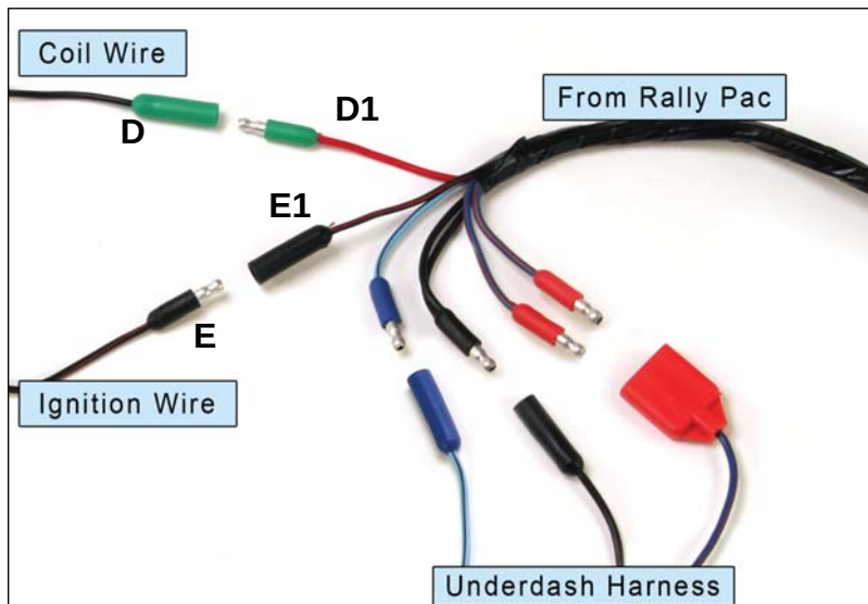
Figure 3: Wiring Diagram
