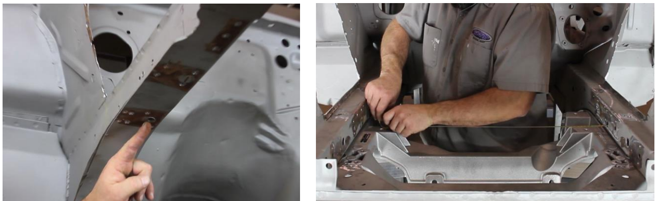
Figure 6 – Locate Aluma-Frame Cradle
