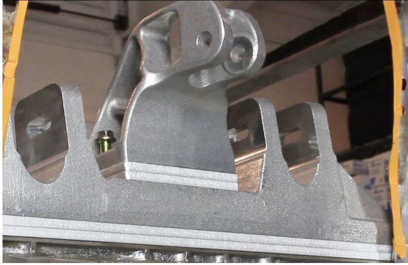
Figure 27 - Install Coilover Mount Shims
