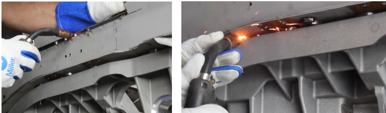
Figure 16 - Tack Weld Adapter Plates & Crush Sleeves
