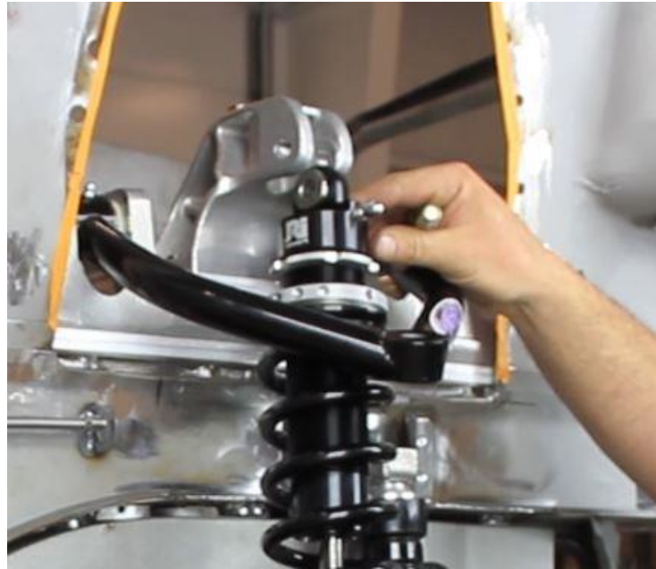
Figure 35 - Upper Coilover Mount
