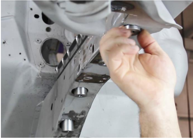
Figure 11 - Install Crush Sleeves
