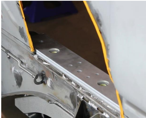
Figure 25 – Install UCA Bracket Shims
