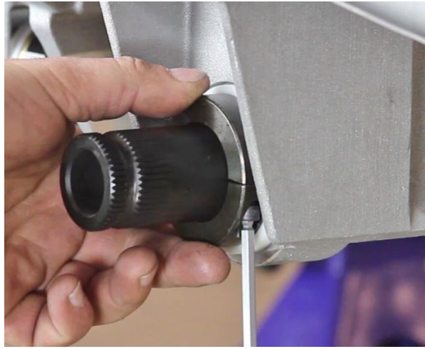
Figure 24 – Install Split Lock Collars
