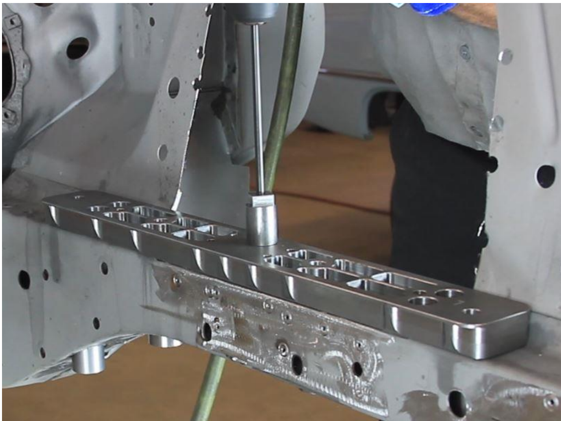
Figure 12 - Locate Coilover Crush Sleeve
