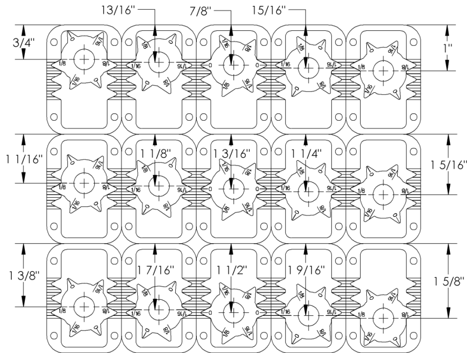
Figure 52 - Detroit Speed Speed-LIGN
