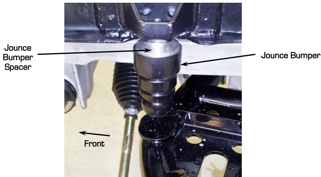
Figure 21 – Install Jounce Bumper
