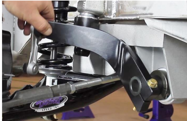
Figure 44 - Install ARB arms
