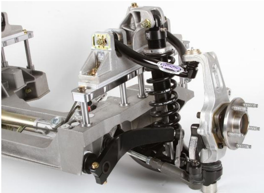
Figure 45 - Fully Assembled View (Driver side, Front)
