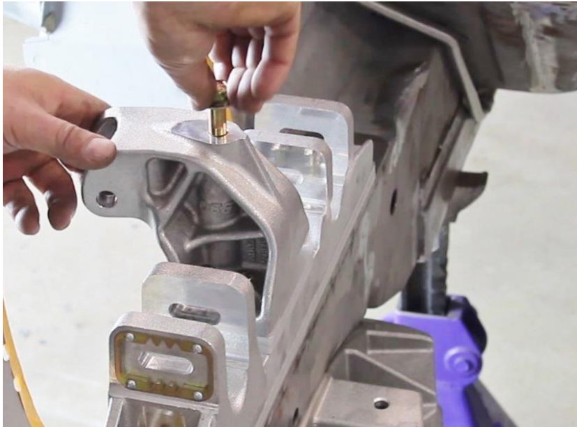
Figure 28 - Install Coilover Mount Brackets
