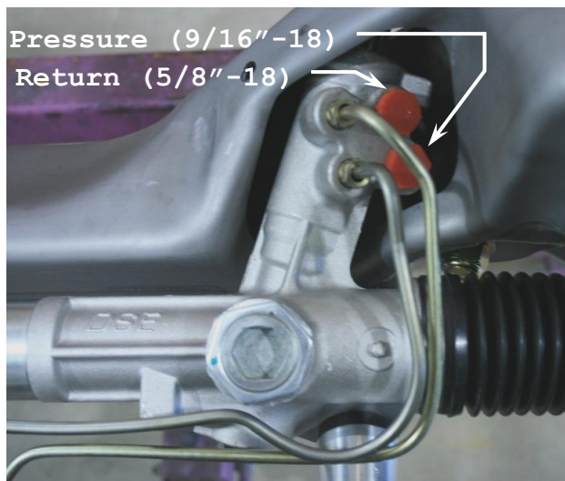
Figure 46 - Pressure and Return Port Locations
