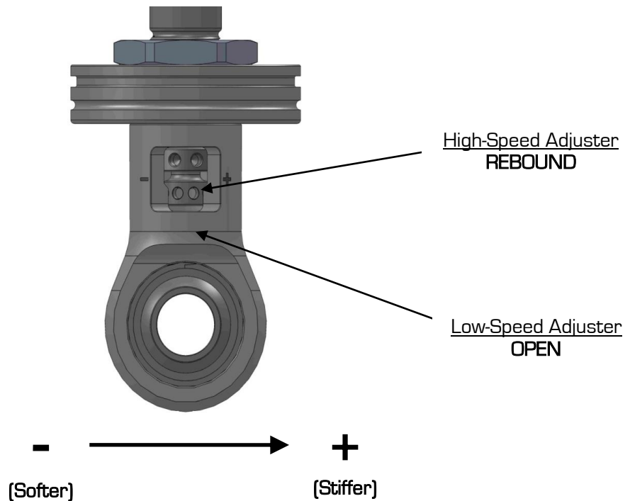
Figure 50b - Detroit Speed Recommended Settings
