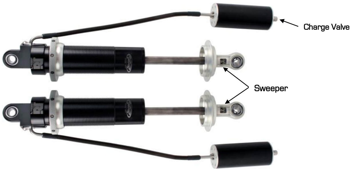
Figure 50a - Detroit Speed Double Adjustable Shock with Remote Canisters
