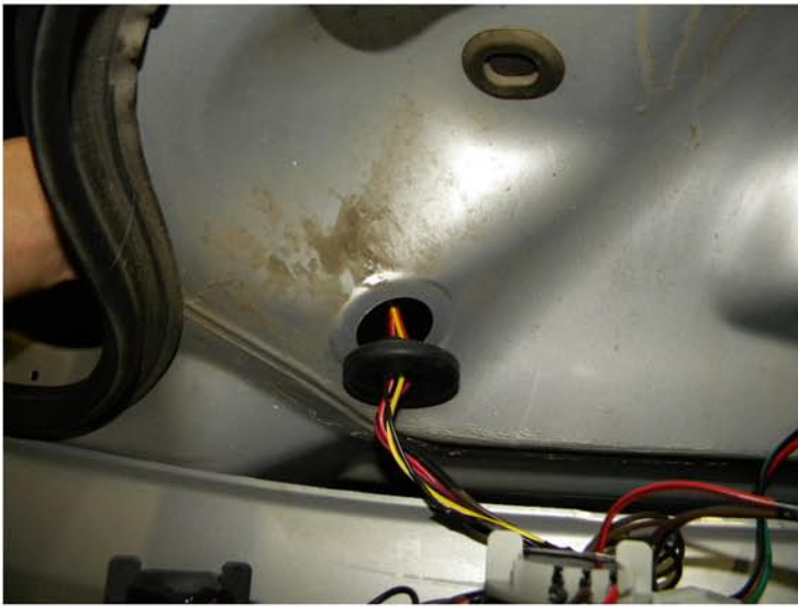
11. Run Tail light harness through body work
