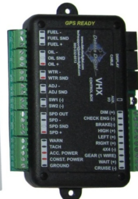
Control Box
