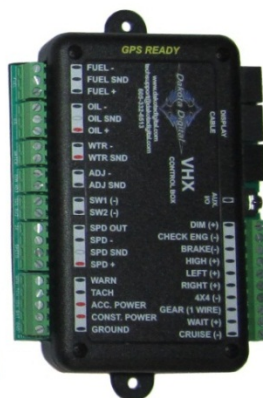
Control Box
